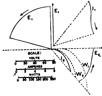
FIG. 16.—Constant Potential, Step Up, Arm at 70°.
